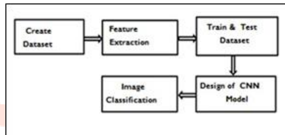
Fig 5.Classifier Flowchart
