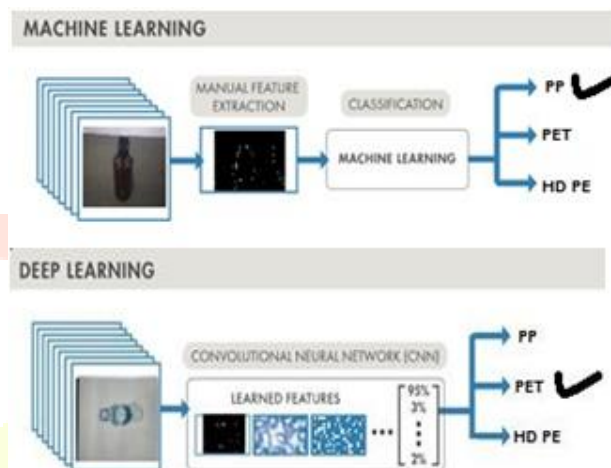
Fig. 3.Feature Extraction on Learning Techniques
