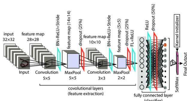
Fig 4.Design of CNN Model
